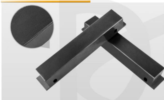
Flat Thread Rolling Die Specialized for Spline Gear Rolling Machine
