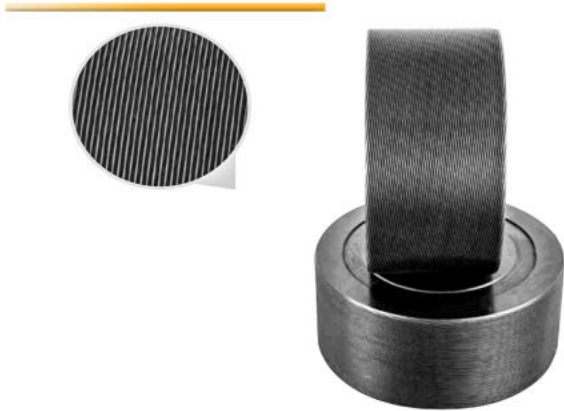
Through Feed Cylindrical Thread Rolling Die for Set Screw
