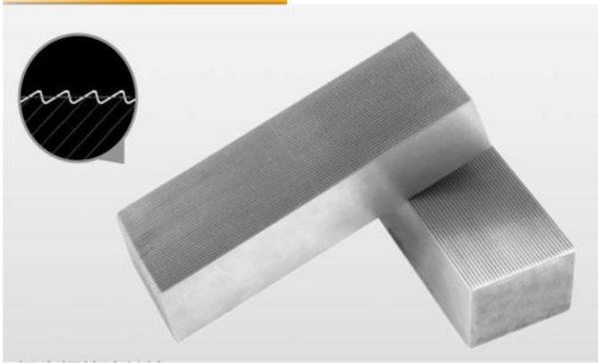
Flat Thread Rolling Die for Buttress Thread
