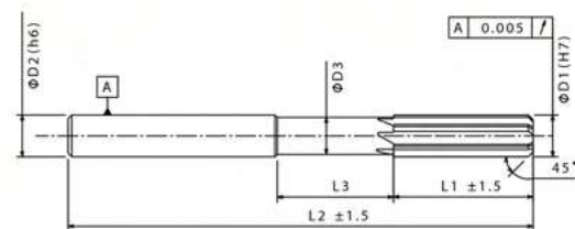
Straight Flute
