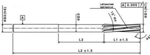
Spiral Flute
